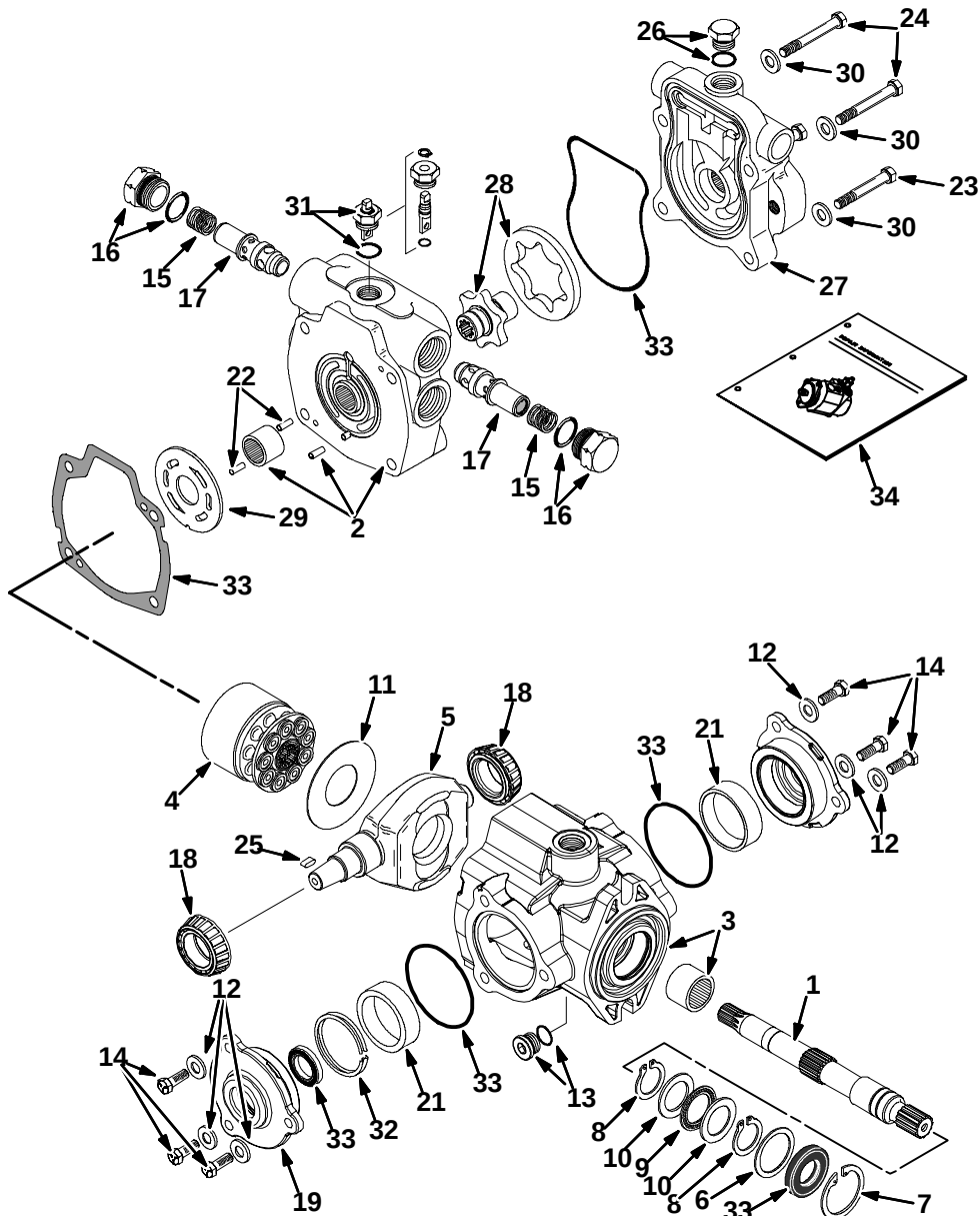
FIG. 1 - HYDRAULIC PISTON PUMP BREAKDOWN, 373387
